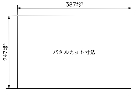
3-1-3 APL4-156BN
