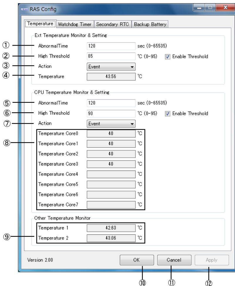
図 2-12-3-1. Temperature Configuration
